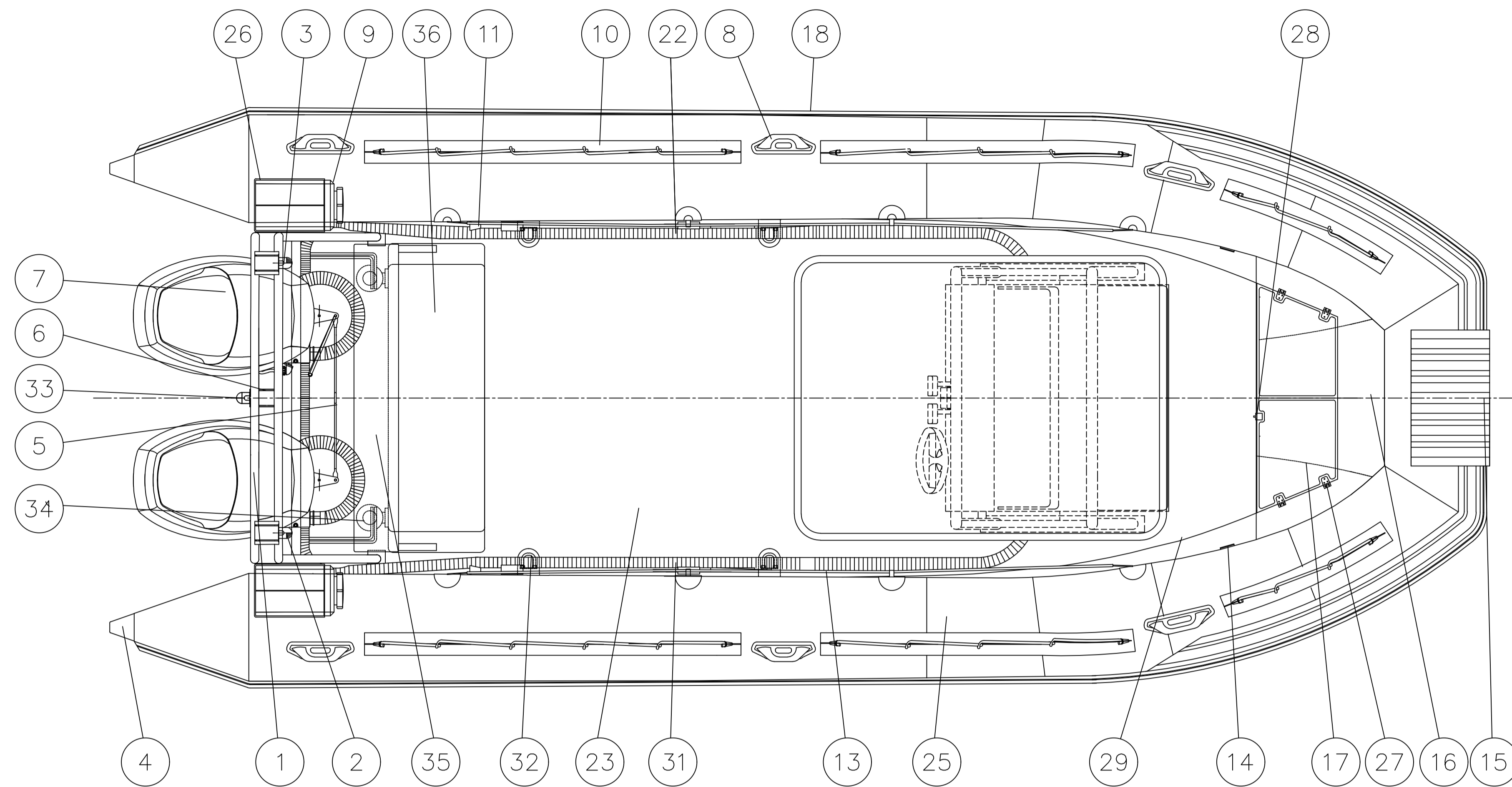
PLAN VIEW WITH BIMINI
