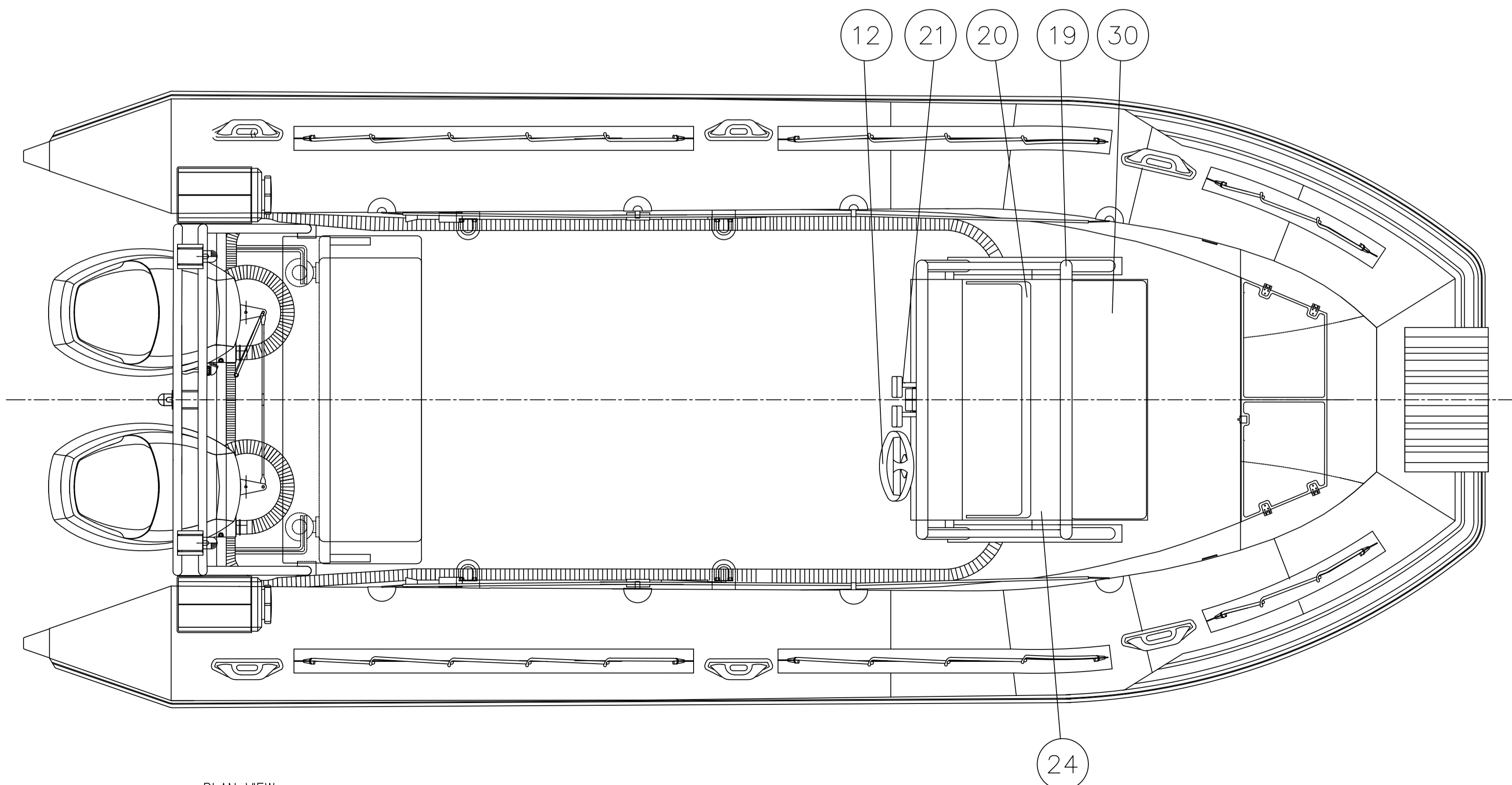
PLAN VIEW WITHOUT BIMINI
